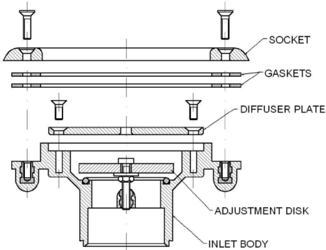
PROPOSED INLET N.T.S.
