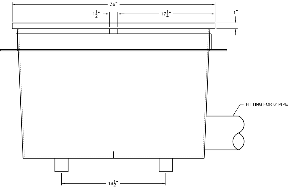
SIDE VIEW - SUMP
