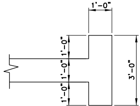
LANE LINE DETAIL
