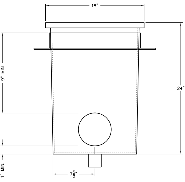
END VIEW - SUMP
