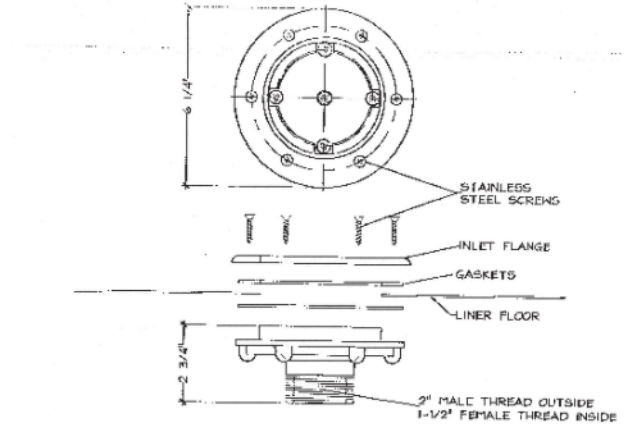
FLOOR LINER INLET:
