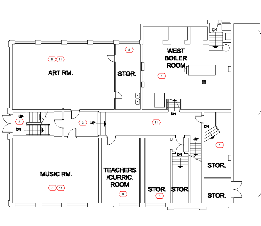
1 ASBESTOS ABATEMENT BASEMENT PLAN NOT TO SCALE
