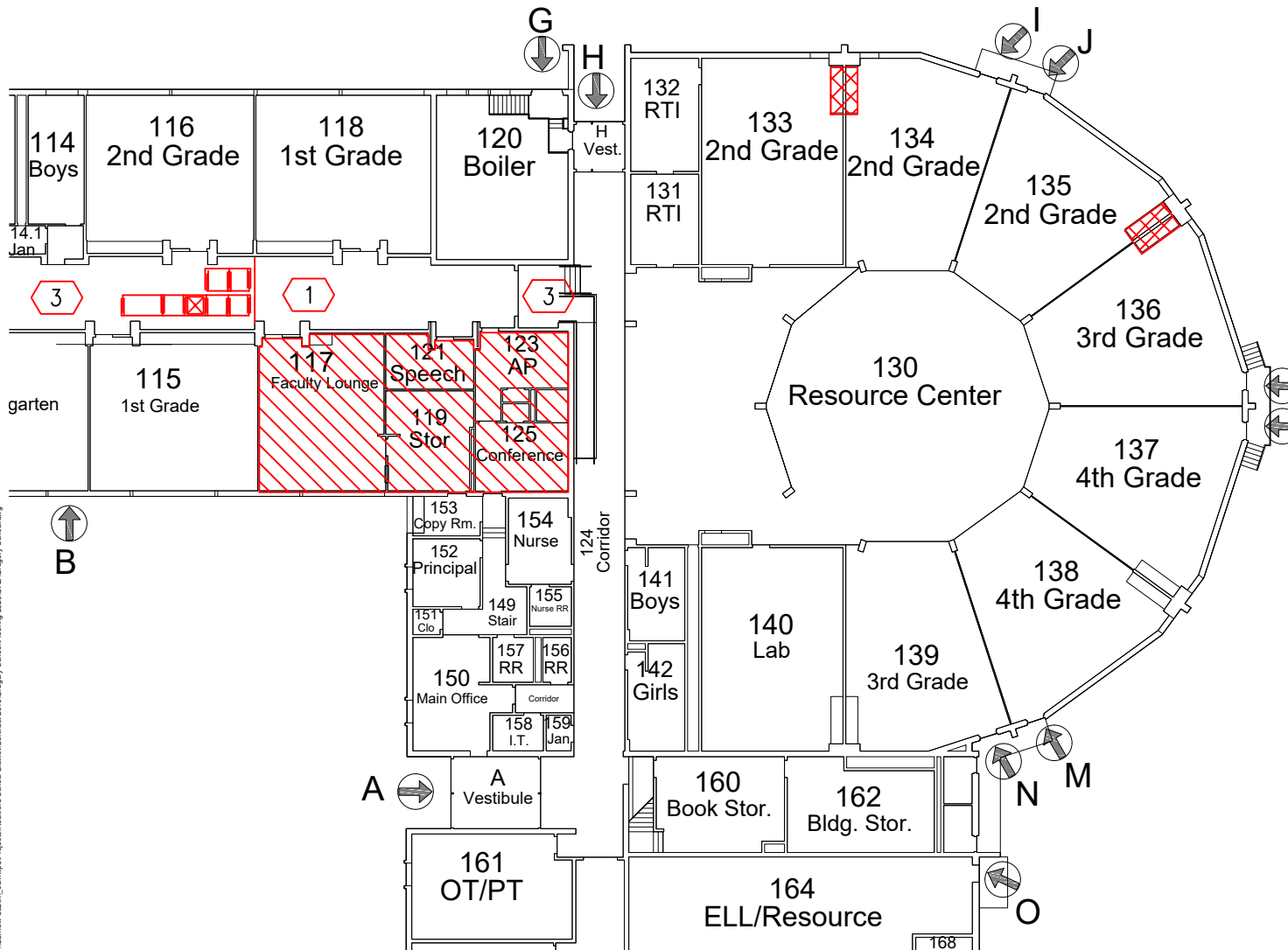
FIRST FLOOR PARTIAL PLAN: ASBESTOS ABATEMENT
