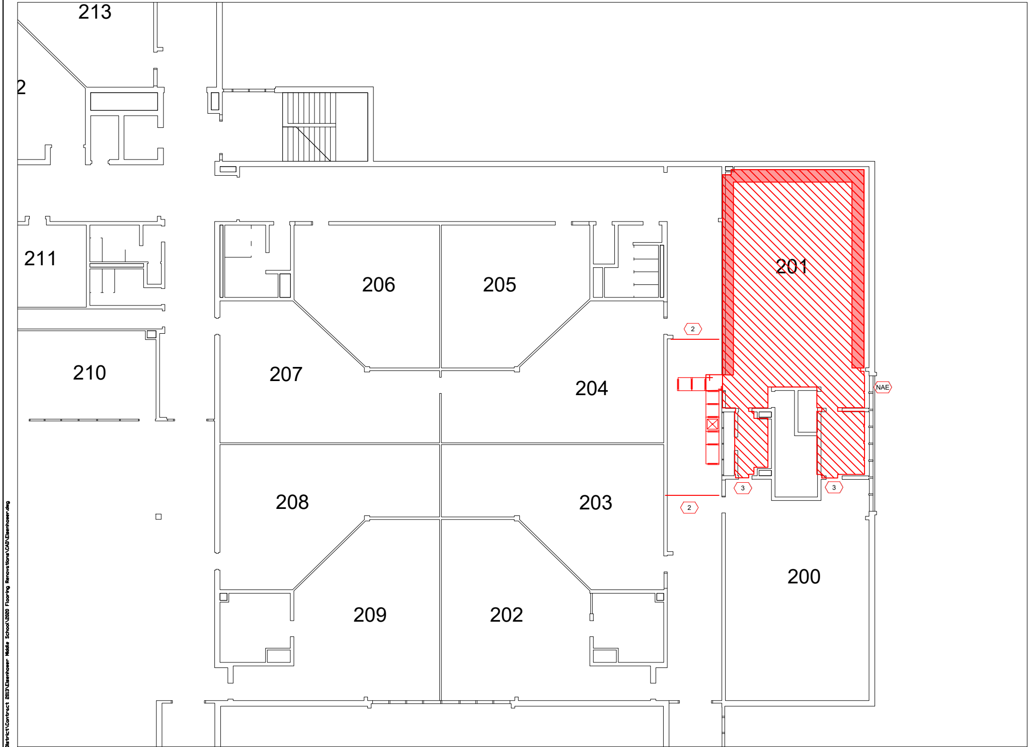
1 ASBESTOS ABATEMENT PARTIAL SECOND FLOOR PLAN NOT TO SCALE
