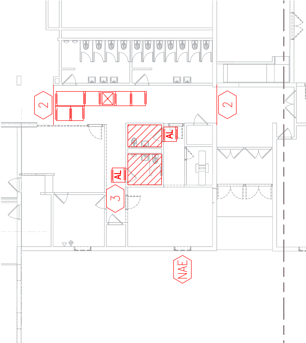
FIRST FLOOR PARTIAL PLAN: ASBESTOS ABATEMENT
