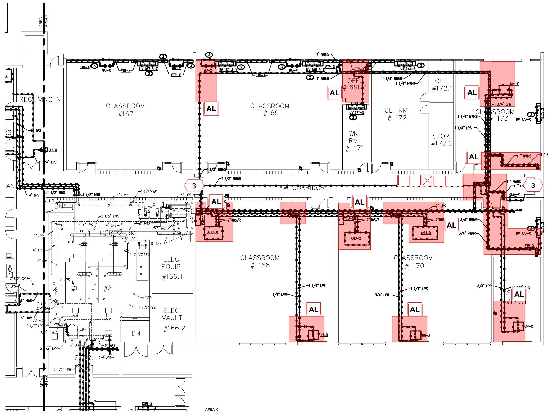
1 ASBESTOS ABATEMENT FIRST FLOOR PLAN
