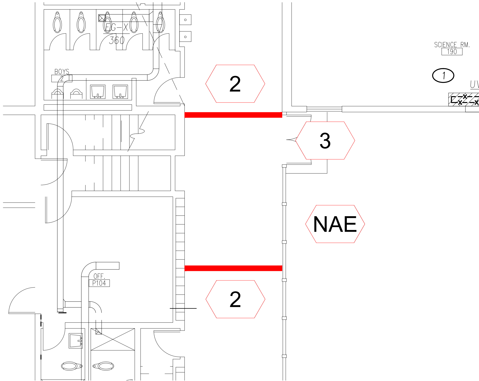
1 ASBESTOS ABATEMENT FIRST FLOOR PARTIAL PLAN
