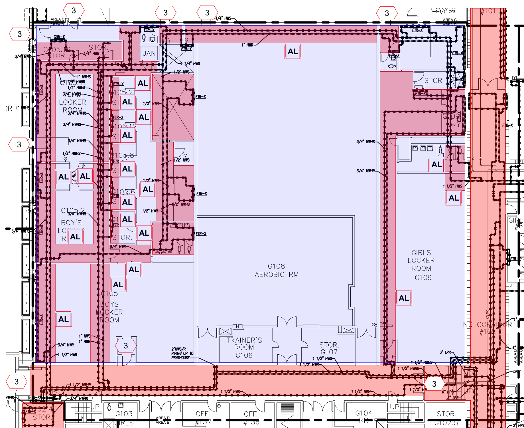
1 ASBESTOS ABATEMENT FIRST FLOOR PLAN
