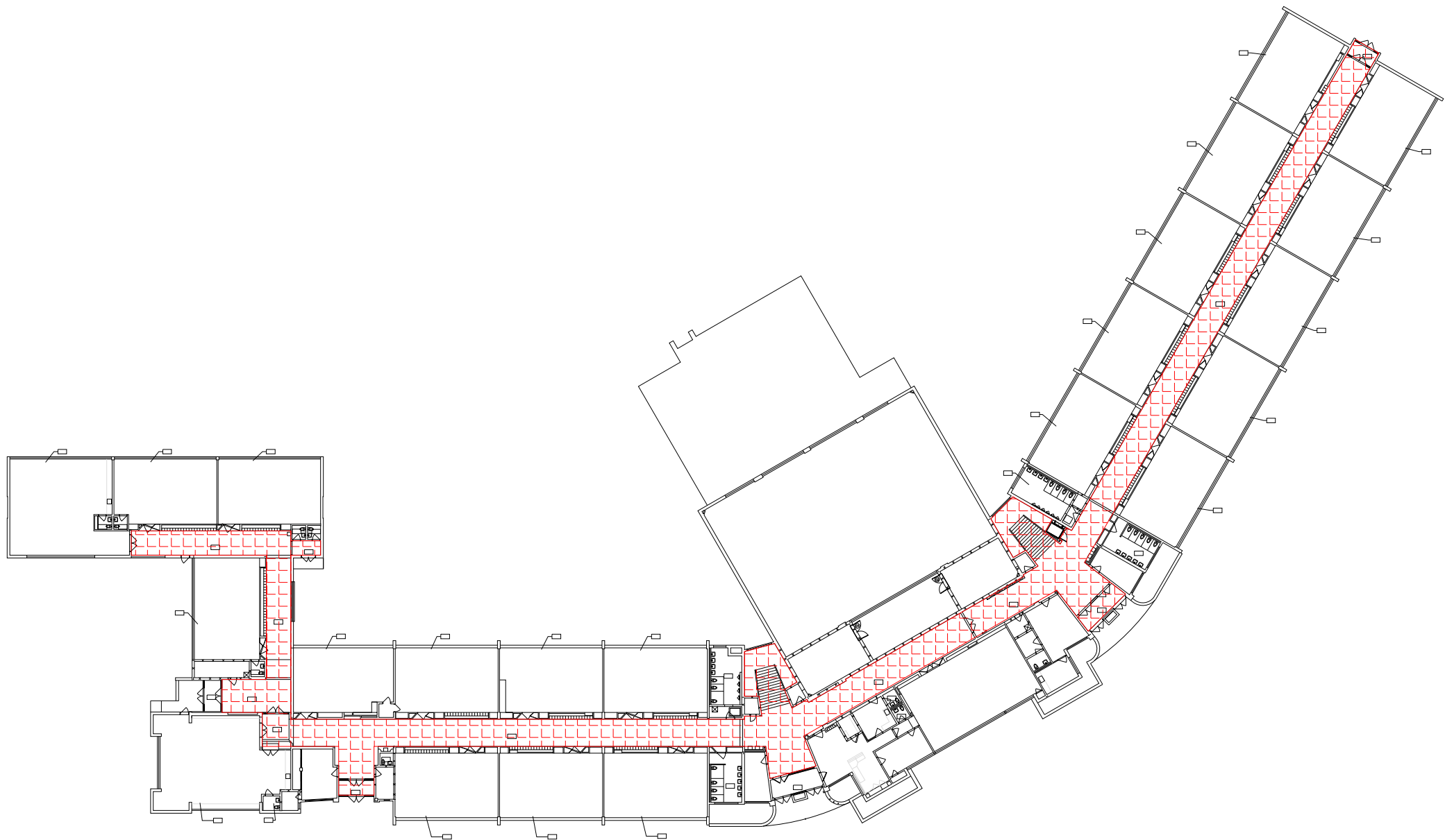
1 GENERAL DEMOLITION FIRST FLOOR PLAN NOT TO SCALE
