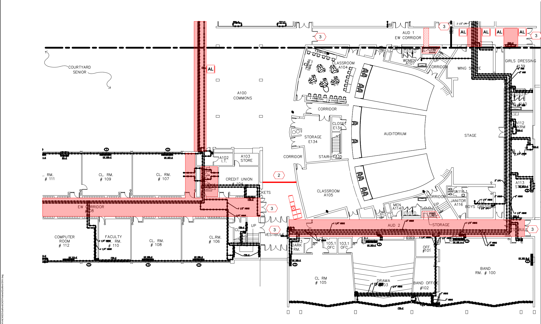
1 ASBESTOS ABATEMENT FIRST FLOOR PLAN NOT TO SCALE N
